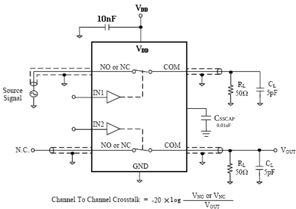
Figure 4, Channel-to-Channel Crosstalk
