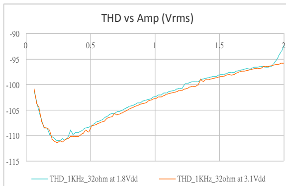
Figure 9, THD vs signal amplitude
